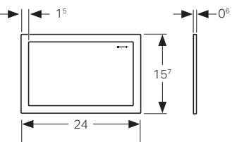
Sigma 60 cover frame
